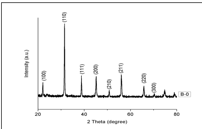
Fig. 2: XRD of pristine BaTiO 3
