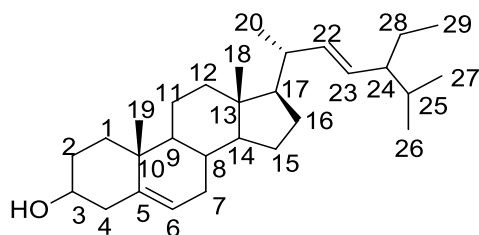
Stigmasterol
