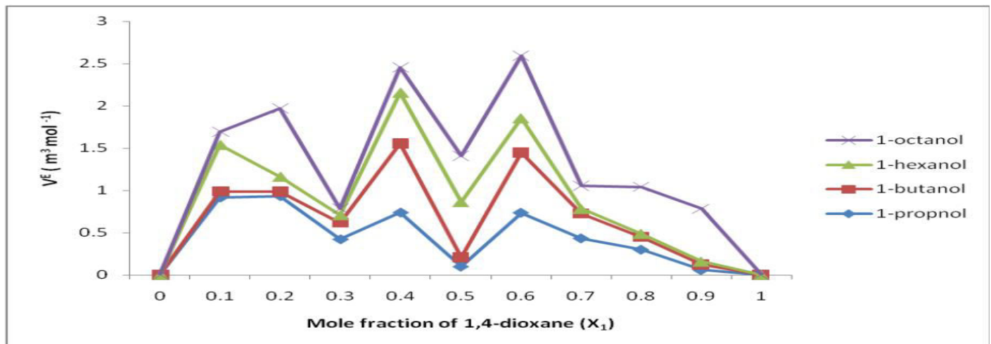
Fig. 1: Plots of excess molar volume ( V^E ) versus mole fraction of 1,4-dioxane ( X_1 ) at 303.15K for binary mixtures of 1,4-dioxane with 1- propanol, 1- butanol, 1-hexanol and 1-octanol
